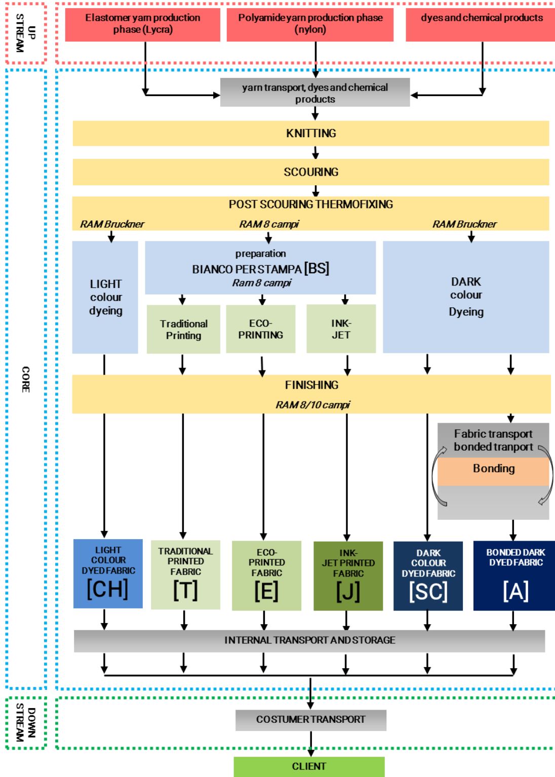
Figure 2-2 Schematic view of system boundaries considered in the PEF study
